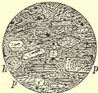
Fig. 35. — Hornblende - Andesite (trachytic type). Summit of Beinn Nevis, Scotland. \times 7 . h , Brown hornblende. p , Plagioclase, often much corroded by the glass around. Fluidal hemicrystalline groundmass.
